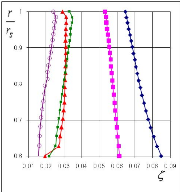
Fig. 6 Total pressure drop in oblique/direct shocks along relative radius. \varphi_s=0,35 . Flow deflection angles 4, 6, 8, 10, 120 from left to right
