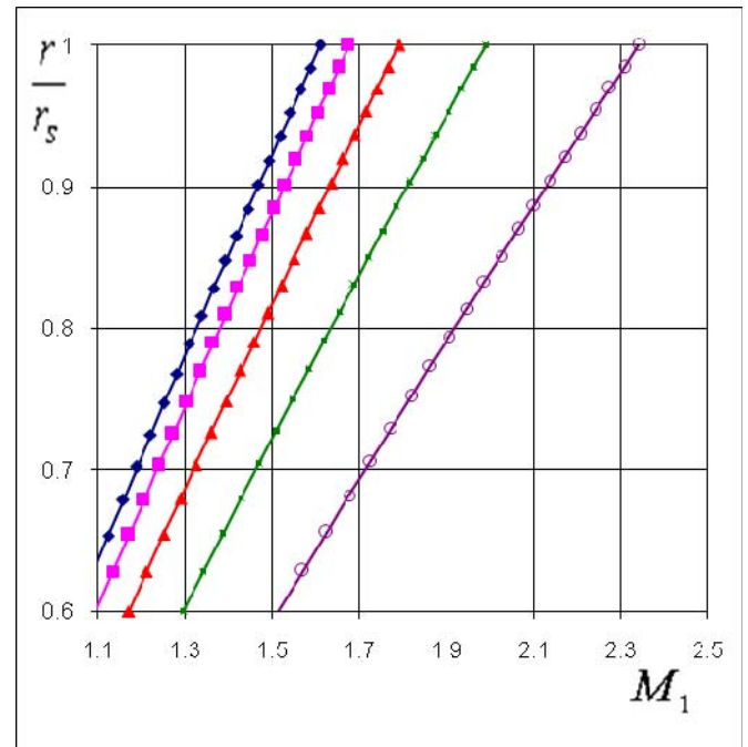
Fig. 5 Inlet Mach number along relative radius. \varphi_s=0,35 .
