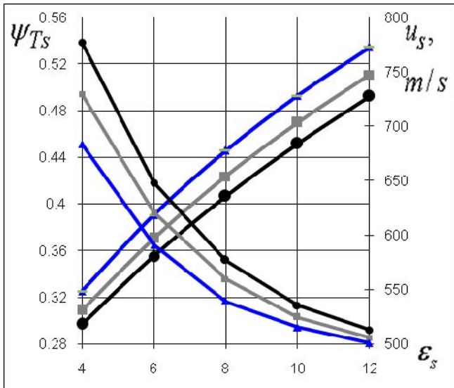
Fig. 3 Periphery blade speed and work coefficient versus periphery deflection angle and flow rate coefficient
